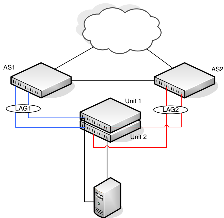
Figure 9-1. Data Center Stack Topology
