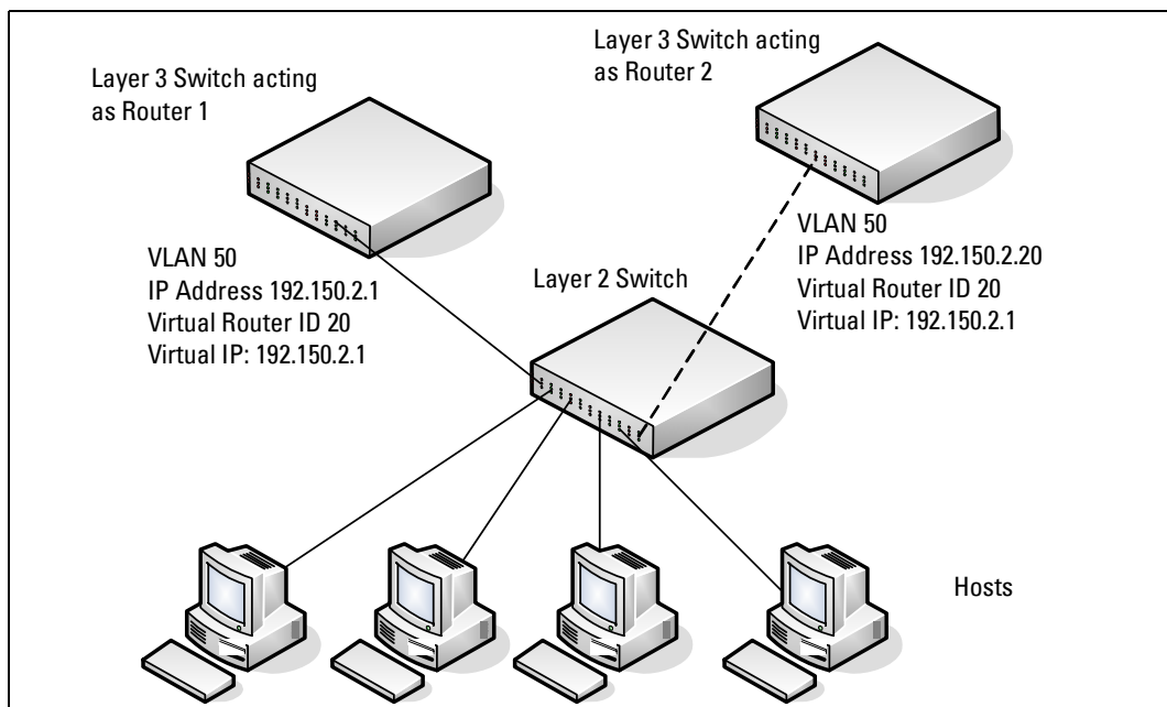
Figure 4-2. VRRP Example Network Configuration
