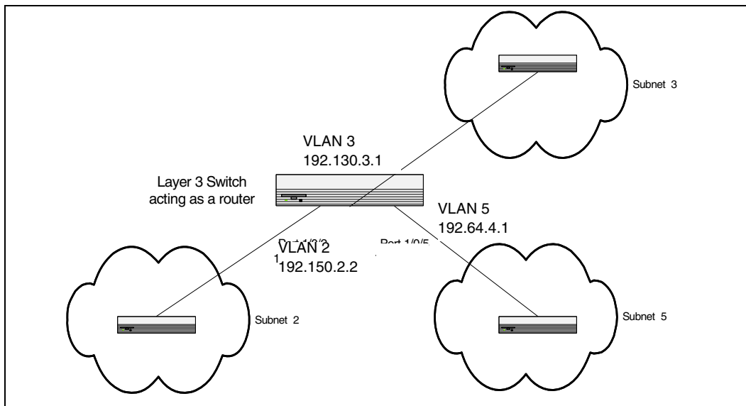
Figure 4-6. Port Routing Example Network Diagram
