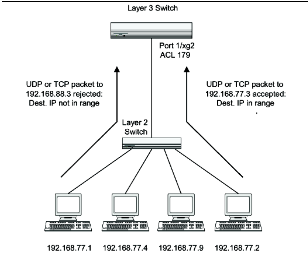
Figure 5-2. IP ACL Example Network Diagram
