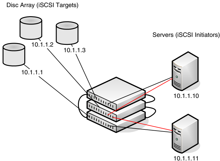
Figure 9-4. NSF and a Storage Area Network
