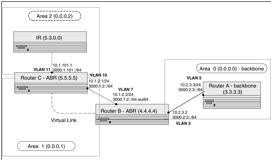
Figure 4-5. OSPF Configuration—Virtual Link
