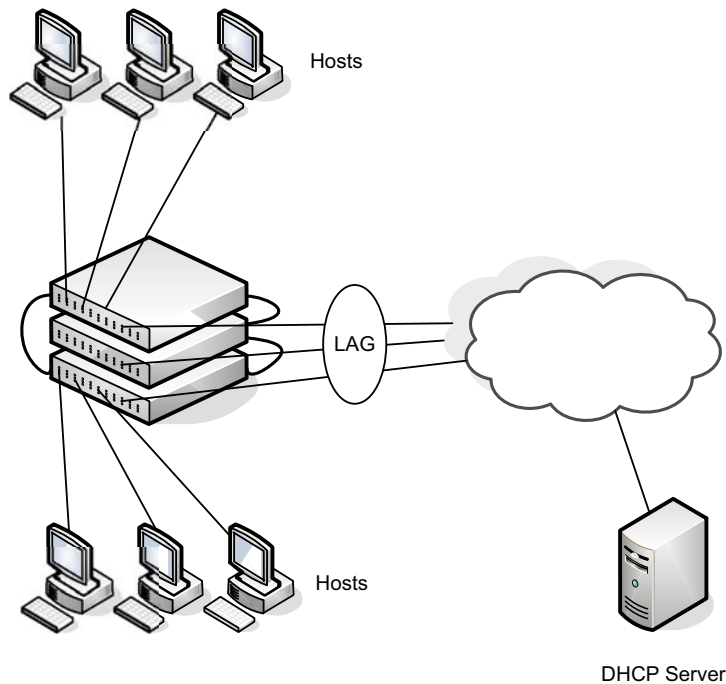
Figure 9-3. NSF and DHCP Snooping
