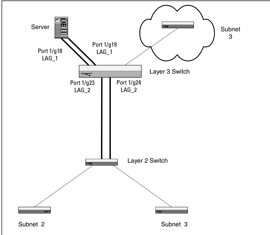
Figure 3-3. LAG/Port-channel Example Network Diagram
