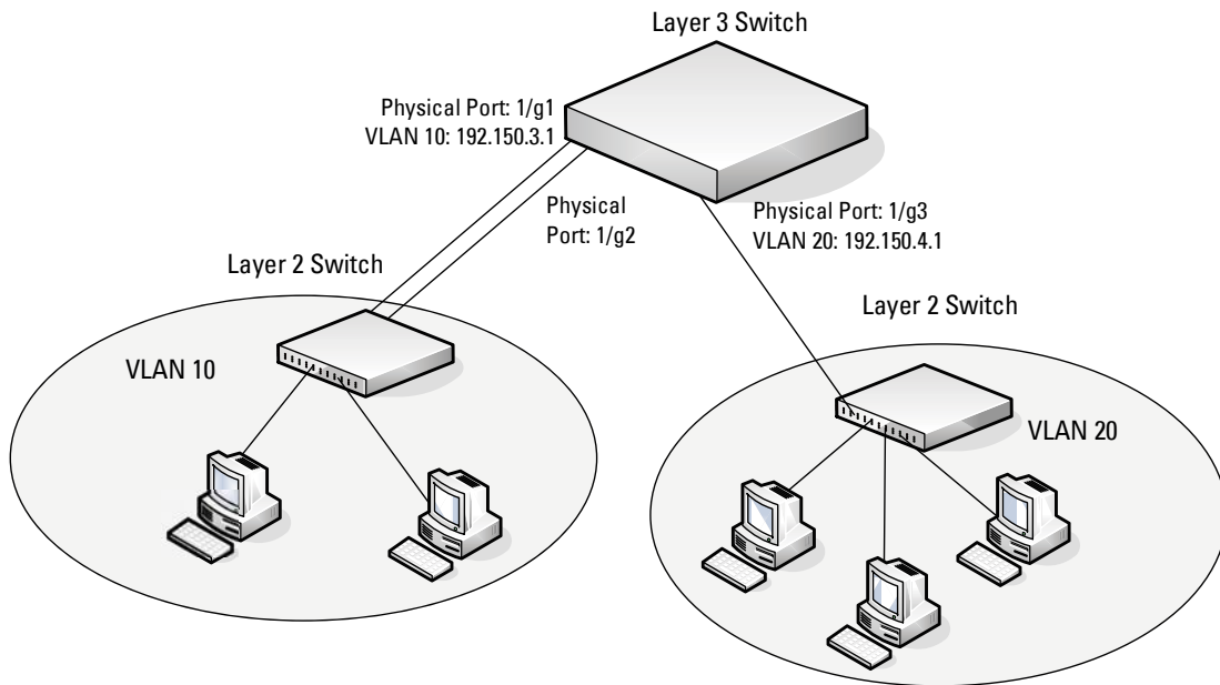
Figure 4-1. VLAN Routing Example Network Diagram
