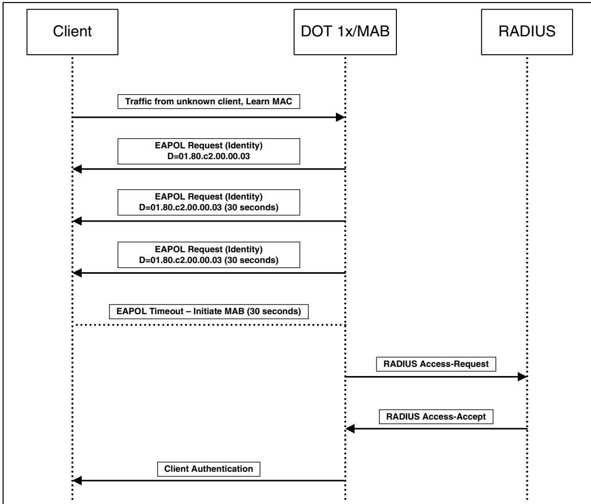
Figure 5-5. MAB Operation – Authentications Based on MAC Address in Database
