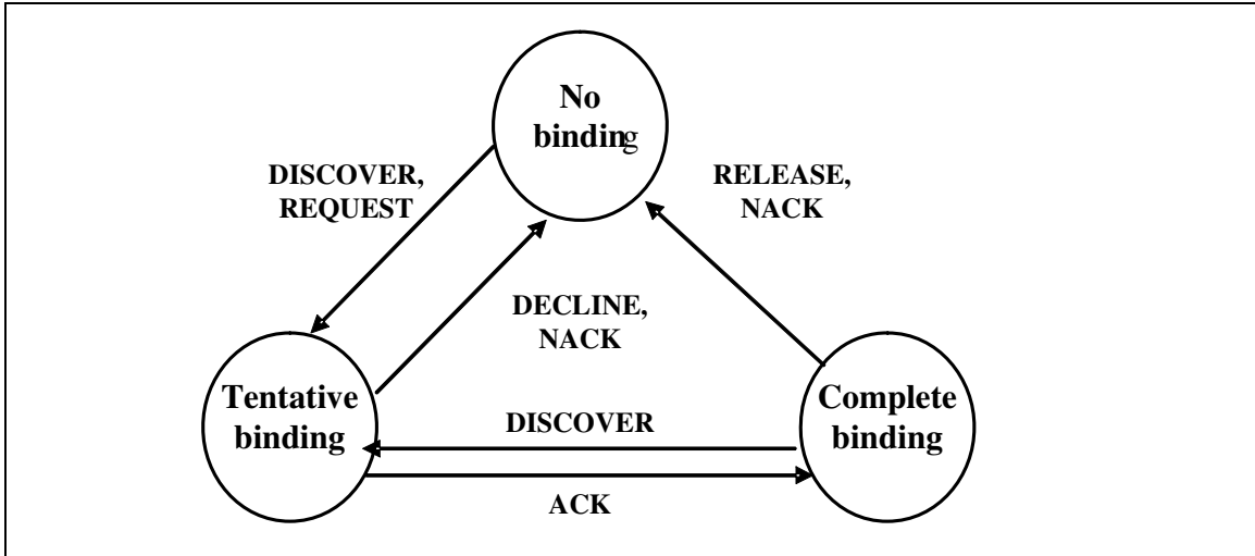
Figure 3-4. DHCP Binding
