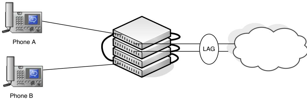
Figure 9-2. NSF and VoIP
