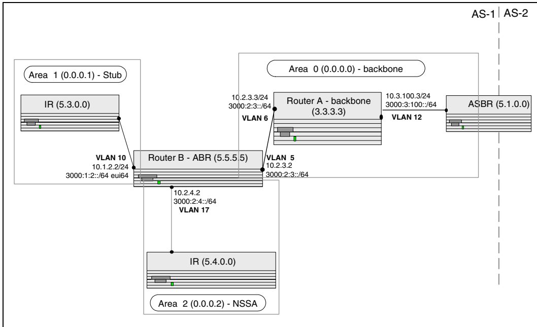
Figure 4-4. OSPF Configuration—Stub Area and NSSA Area
