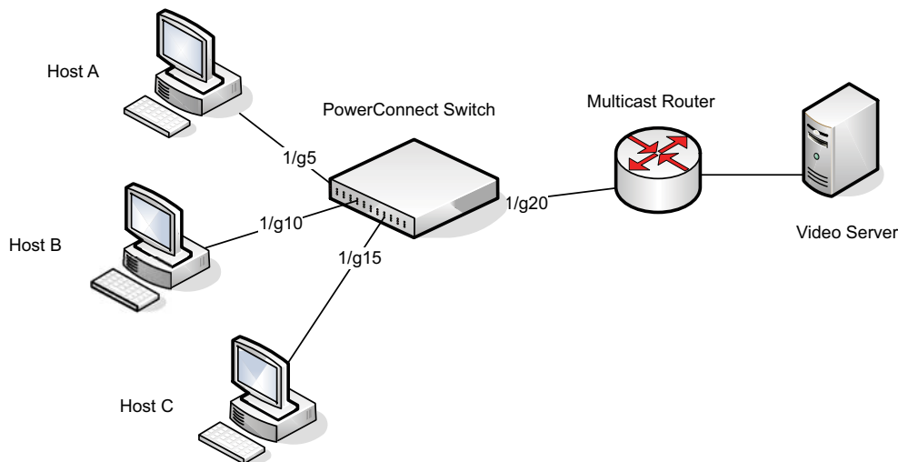
Figure 3-2. Switch with IGMP Snooping
