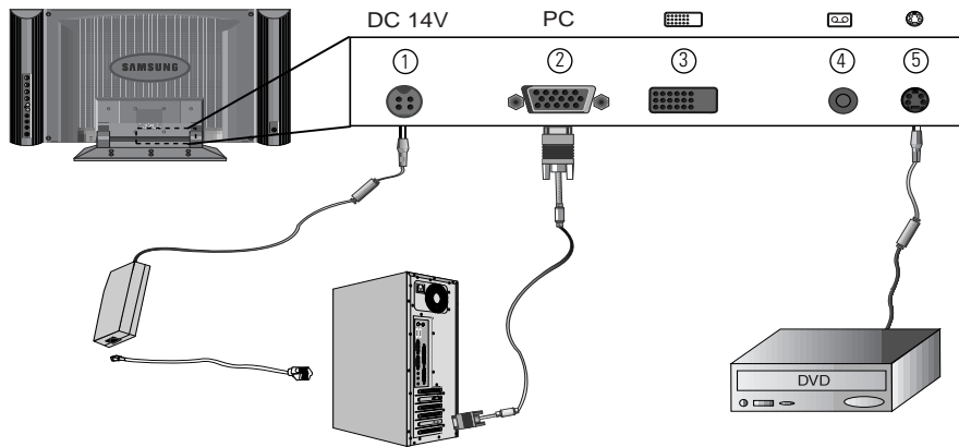
Figure 3. Cable connections
