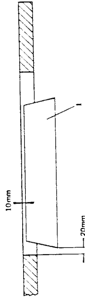
Fig. 1 To attach drip pan to the table
