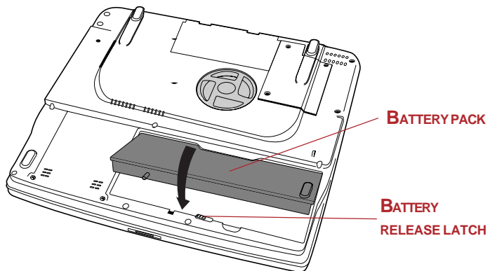
Figure 6-2 Securing the battery pack
