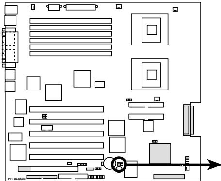
PR-DLS533 Wake-On-Ring Connector
