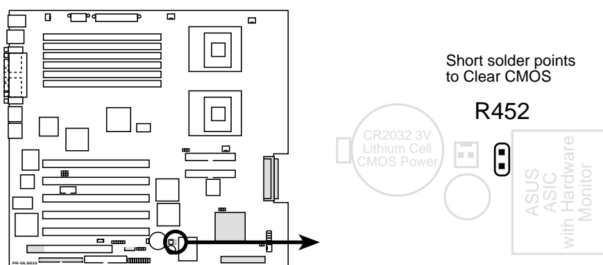
PR-DLS533 Clear RTC RAM
