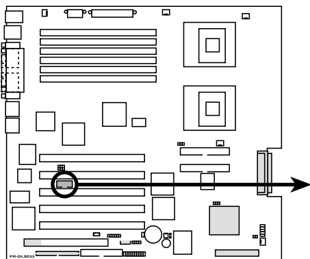
PR-DLS533 Serial COM2 Connector
