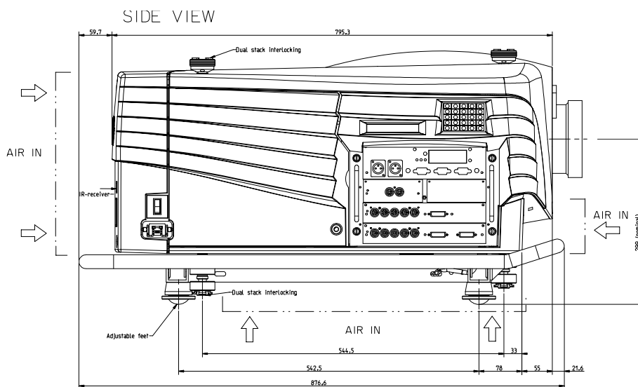
Image 2-3 Side view dimensions
