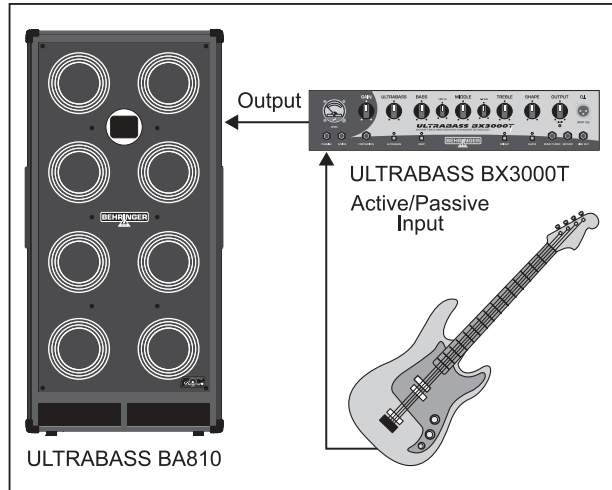
Fig. 3.3: Setup with the BA810 and the BX3000T
