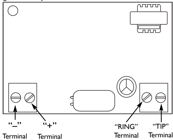
Figure 2 - Amplifier PC Board
