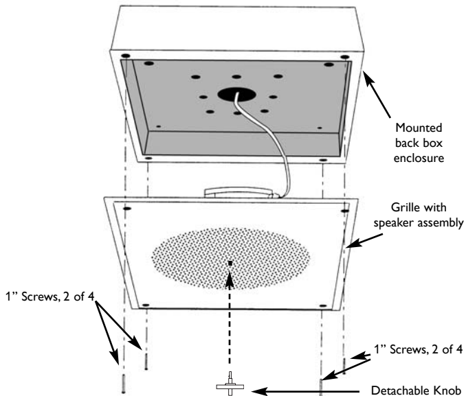
Figure 3 - Secure faceplate
