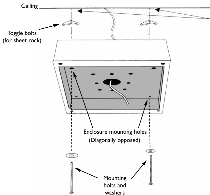
Figure 1 - Sheet rocked ceiling mounting example
