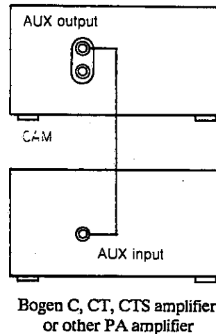
Figure 4 — Single connection for increased inputs
