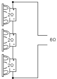
Three 2Ω subs, series
