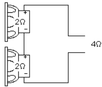
Two 2Ω subs, series
