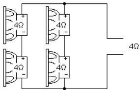
Four 4Ω subs, series/parallel
