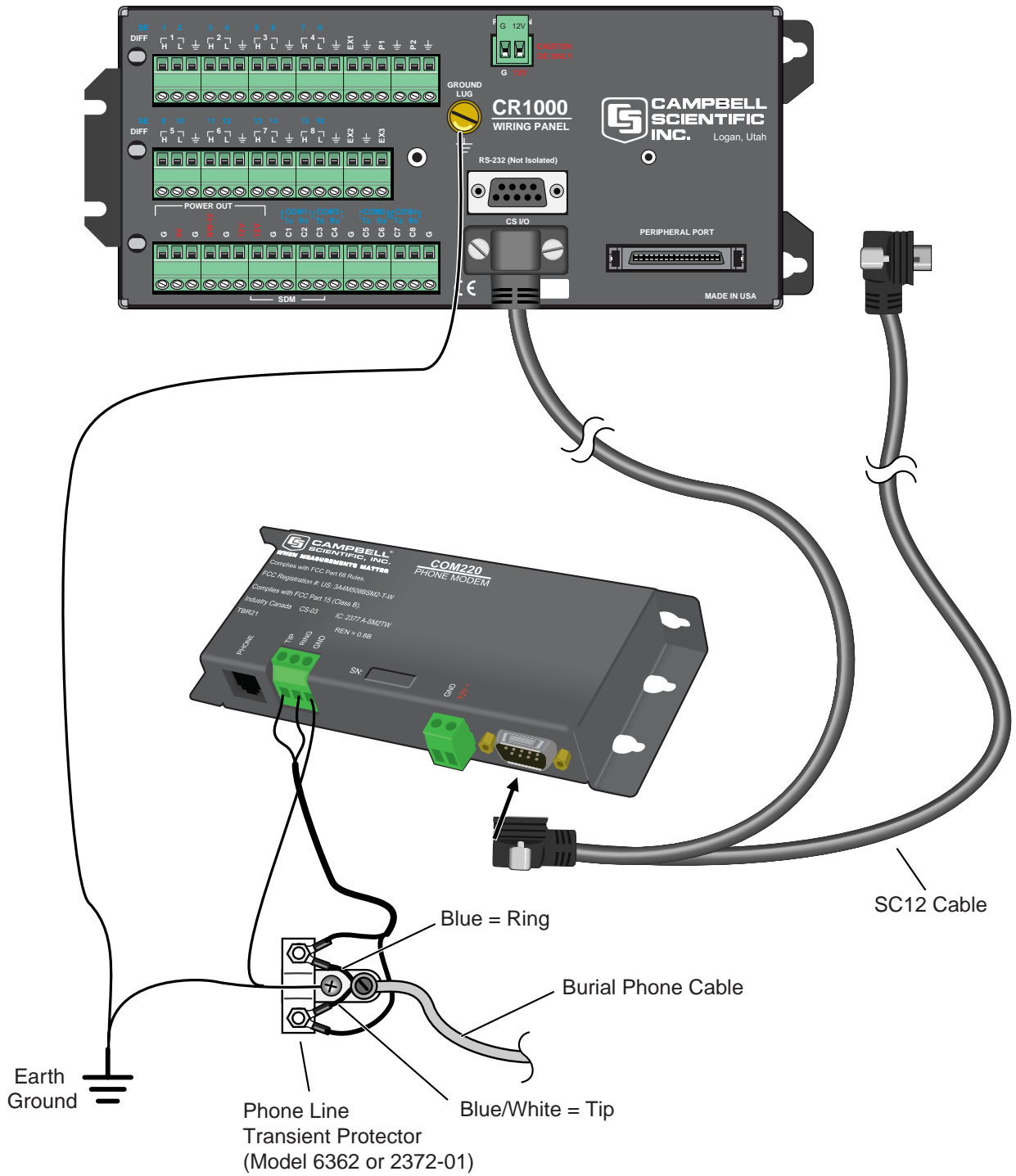
FIGURE 3. CR1000 and COM220 Using Remote Telephone Line
