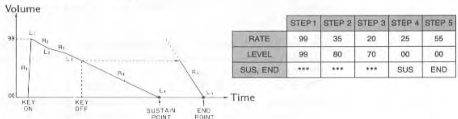
(Fig. 10) Piano amp envelope
