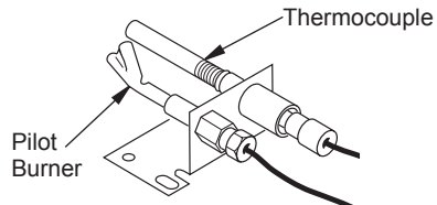
Figure 13 - Thermocouple and Pilot
