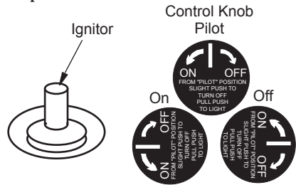
Figure 12 - Ignitor and Control Knob
