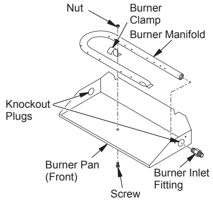
Figure 6 - Installing Burner
